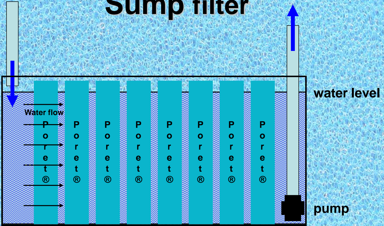
Side view wet sump
